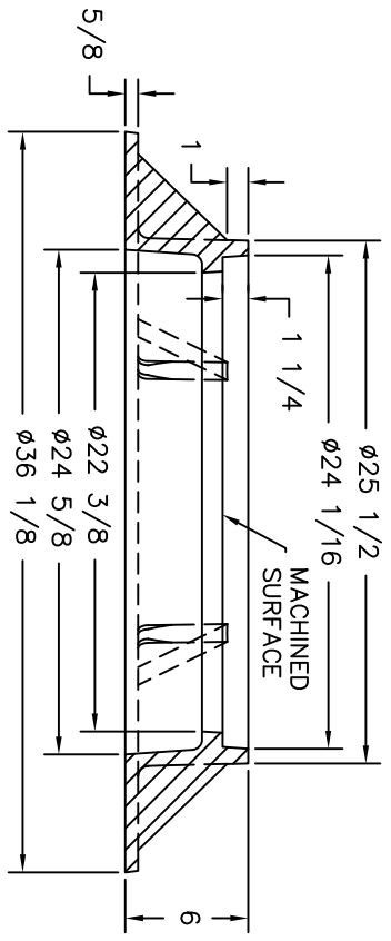
SECTION B-B (Ring)
