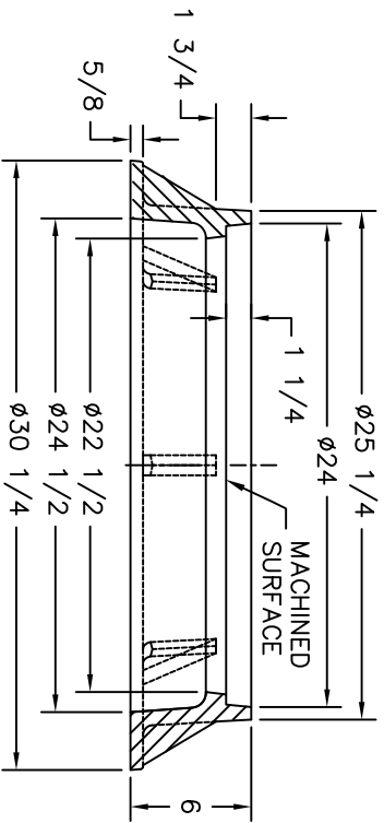
SECTION B-B (Ring)
