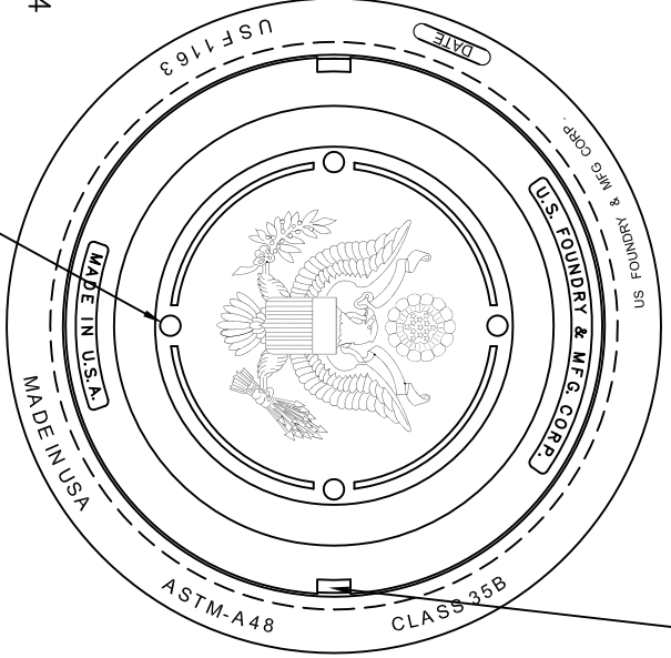
(2) - NON-PENETRATING PICKHOLES
