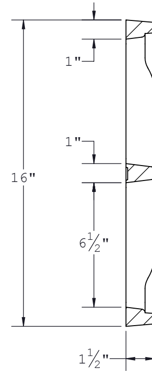
SECTION B-B
