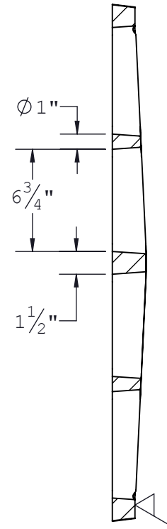
SECTION B-B
